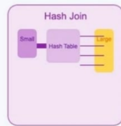
Hash Join
